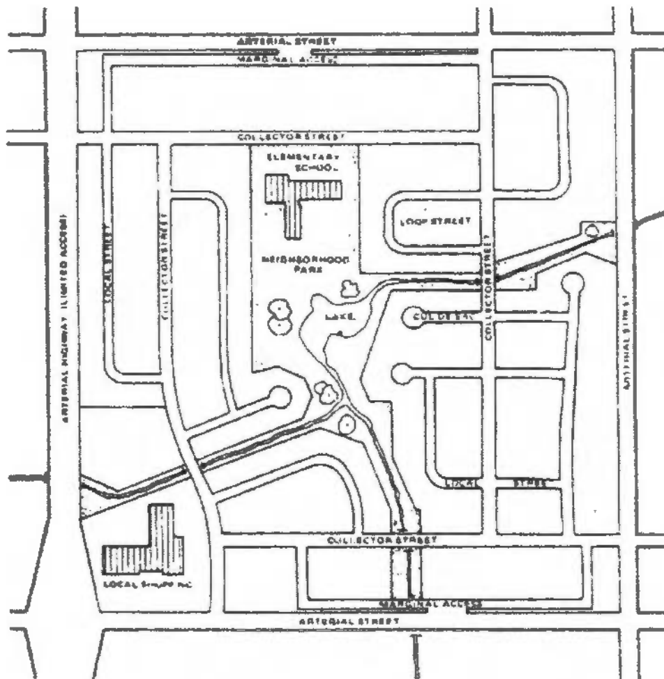
CLASSIFICATION OF THE THOROUGHFARE SYSTEM
